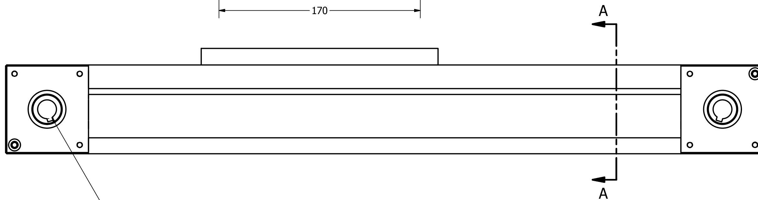
HOLLOW SHAFT -16- WITH KEYWAY (2x)
